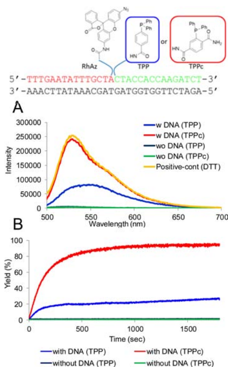
Figure 2. DNA-templated Staudinger reaction by conventional RhAz-TPP or new RhAz-TPPc. (A) Fluorescence spectrum of reaction mixture after 30 min. (B) Time course of DNA-templated Staudinger reaction. Conditions: 100 nM RhAz probe, 300 nM TPP or TPPc probe, 100 nM DNA target in 20 mM Tris-HCl (pH 7.2) containing 100 mM MgCl 2 and 10 μg/mL BSA, 37 °C, 30 min, ex 490 nm, em 525 nm. Yield was calculated from reduced RhAz probe by dithiothreitol (DTT).
